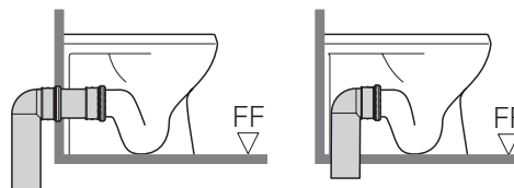
A. Floor-Mount Rear Discharge into Wall
